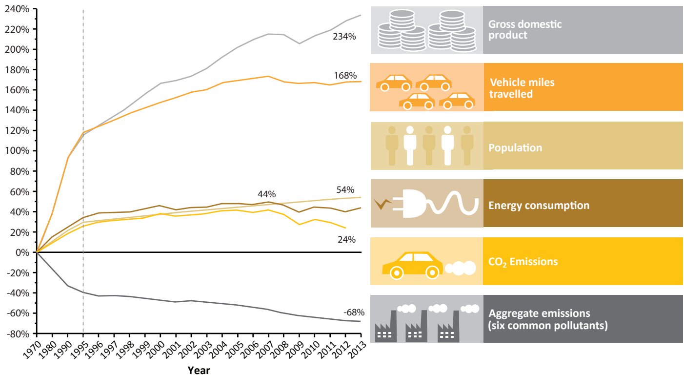
Figure 2.1.1: US trends in drivers and emissions, 1970–2013
