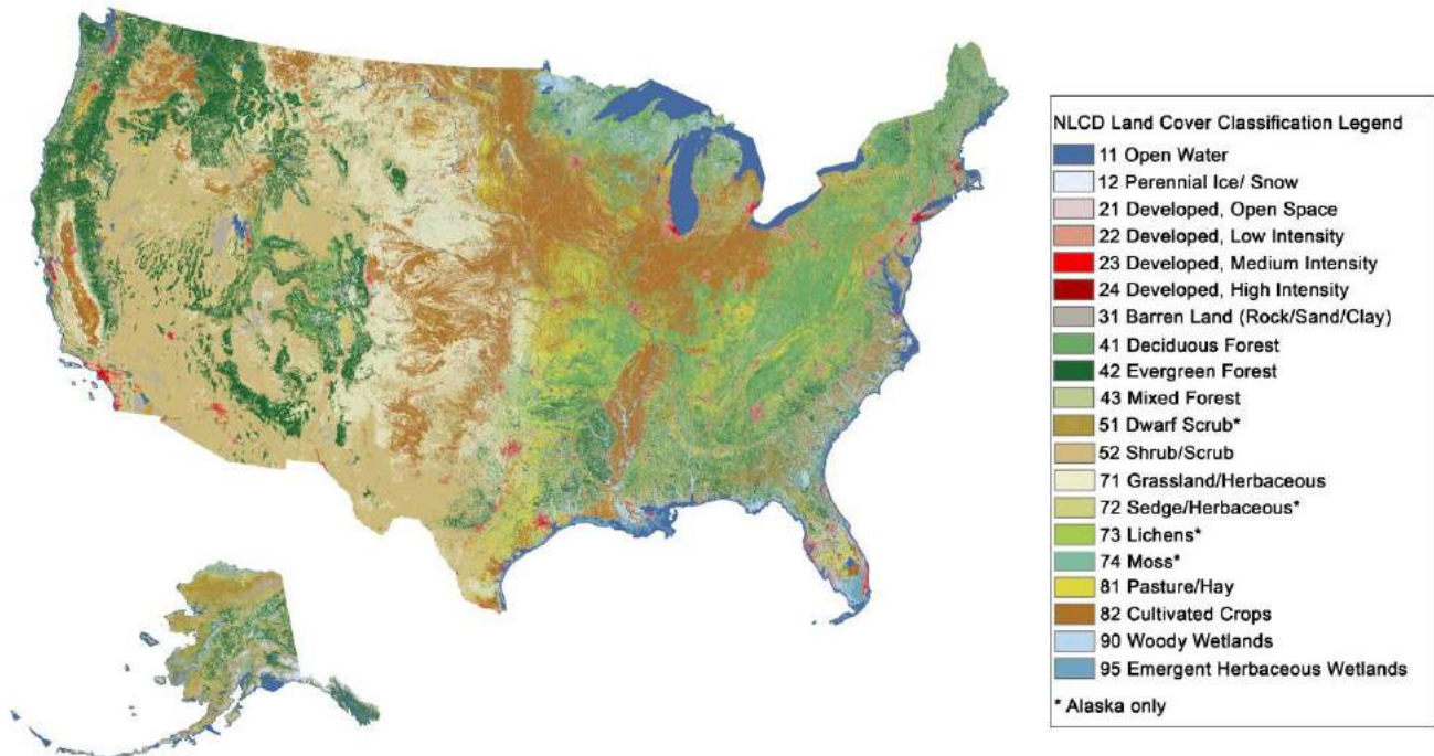
Figure 2.2.6: US land cover, 2011
